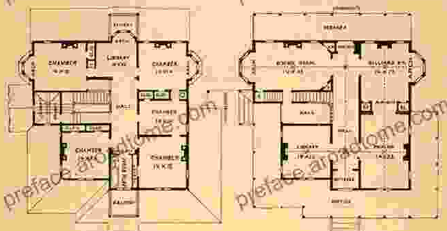
— SECOND FLOOR — — FIRST FLOOR — DESIGN FOR SUBURBAN RESIDENCE, COSTING FROM $5,000 TO $6,000.
